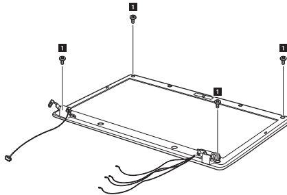
Figure 17. Removal steps of LCD front bezel
