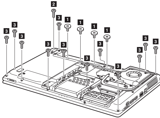
Figure 12. Removal steps of keyboard bezel
