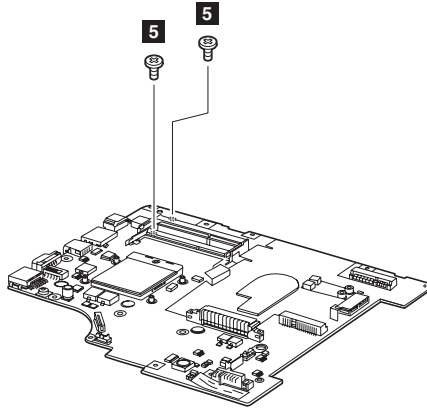
Figure 14. Removal steps of system board and ExpressCard slot assembly (continued)
