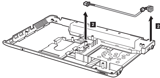
Figure 16. Removal steps of bluetooth daughter card and base cover (continued)
