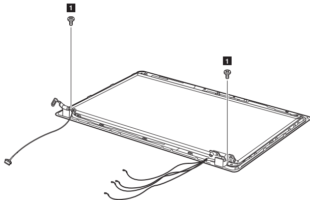
Figure 18. Removal steps of LCD panel and hinges
