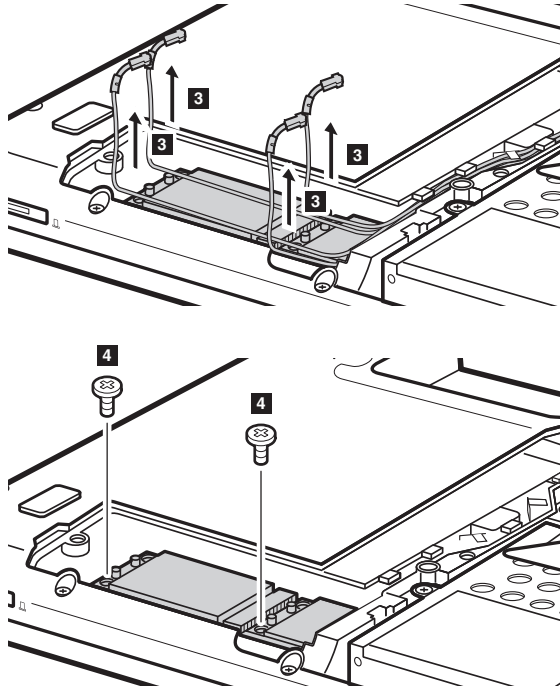
Figure 10. Removal steps of PCI Express Mini Card for wireless LAN/WAN
